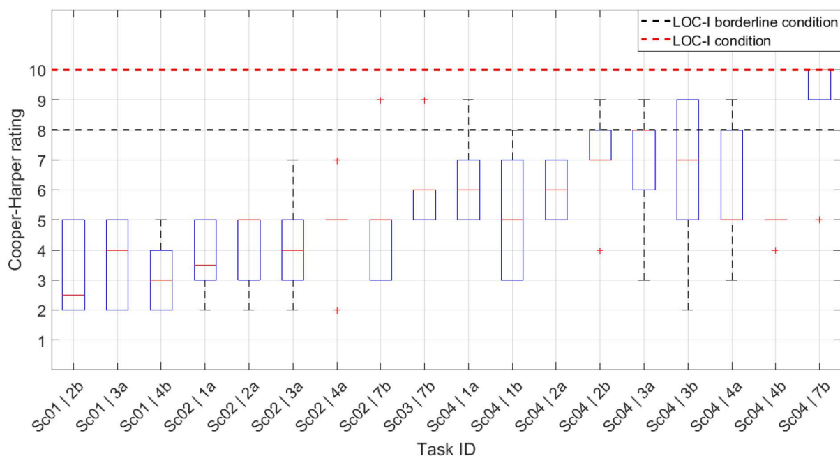
Fig. 6 Cooper-Harper ratings.
