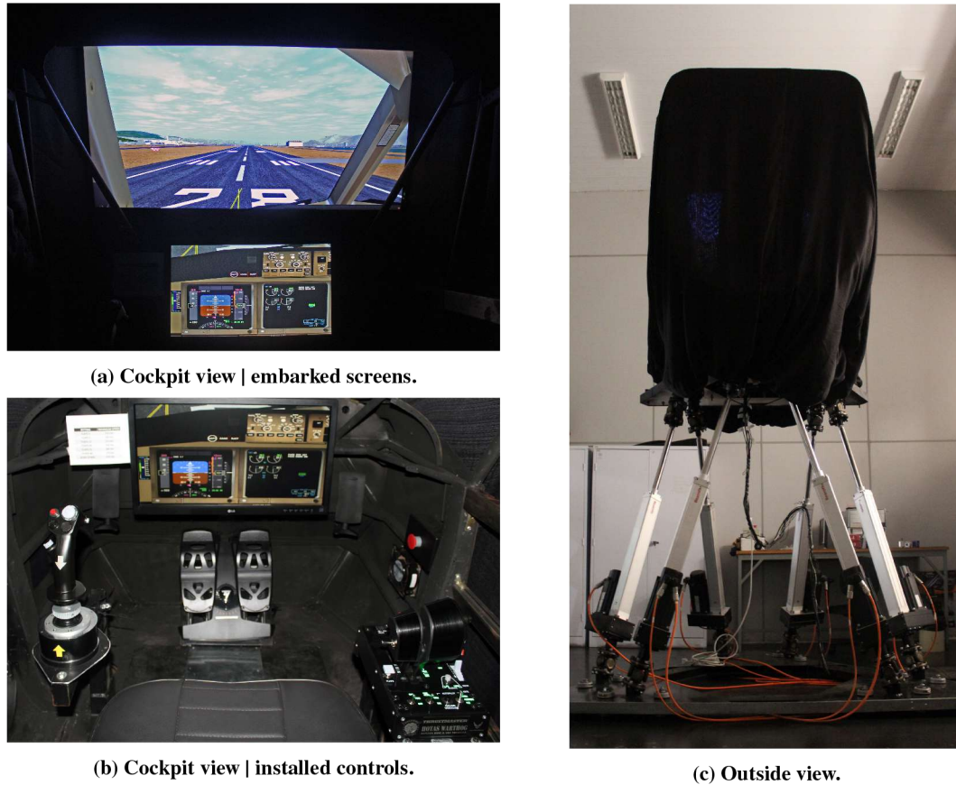
Fig. 4 EESC-USP's flight simulator.
