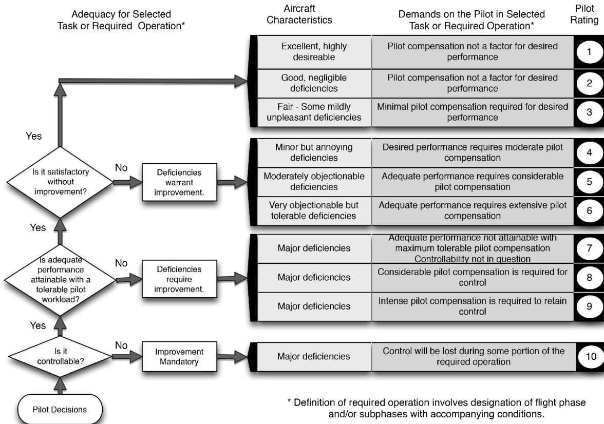
Fig. 2 The Cooper-Harper rating scale – adapted from [14].
